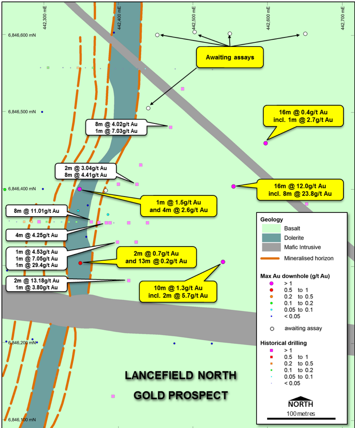
Figure 2. Plan View of the Lancefield North Prospect.
