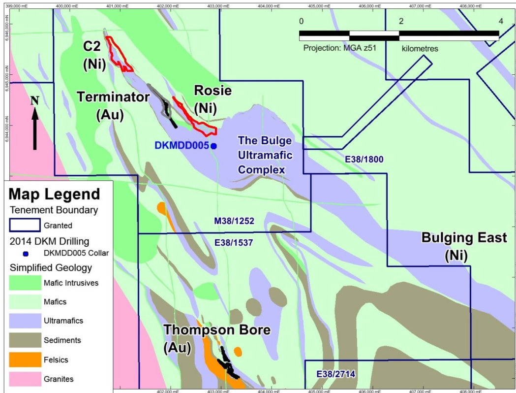
Figure 2: Plan showing collar location of DKMDD005
