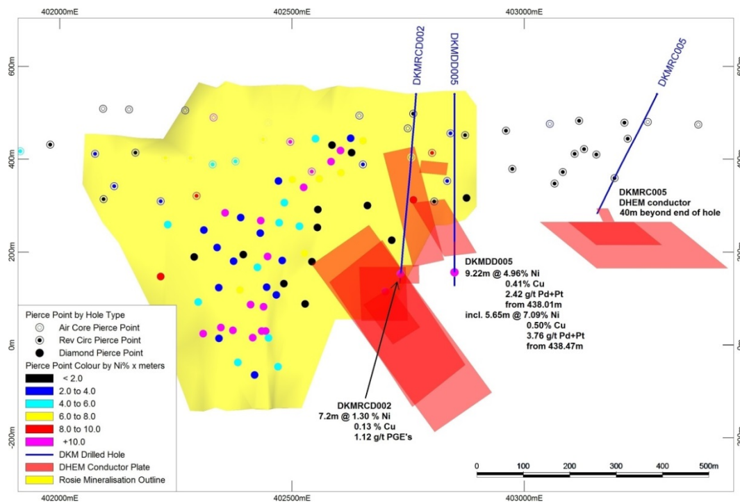
Figure 3: Long-section looking north showing the Rosie mineralisation in yellow, DKMDD-005 and the relevant DHEM plates in red.
