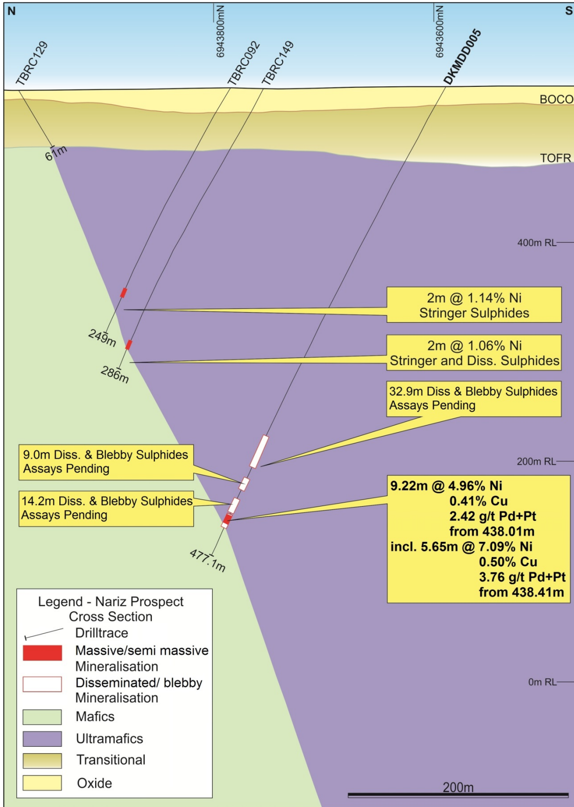
Figure 4: Interpreted cross-section looking east showing DKMDD-005. TBRC129. TBRC092 and TBRC149 are historical drill holes.
